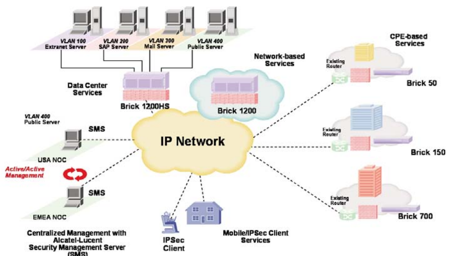
The Alcatel-Lucent VPN Firewall Brick portfolio offers flexible deployment options to suit enterprise, government, and service provider network strategies and users' diverse needs.
